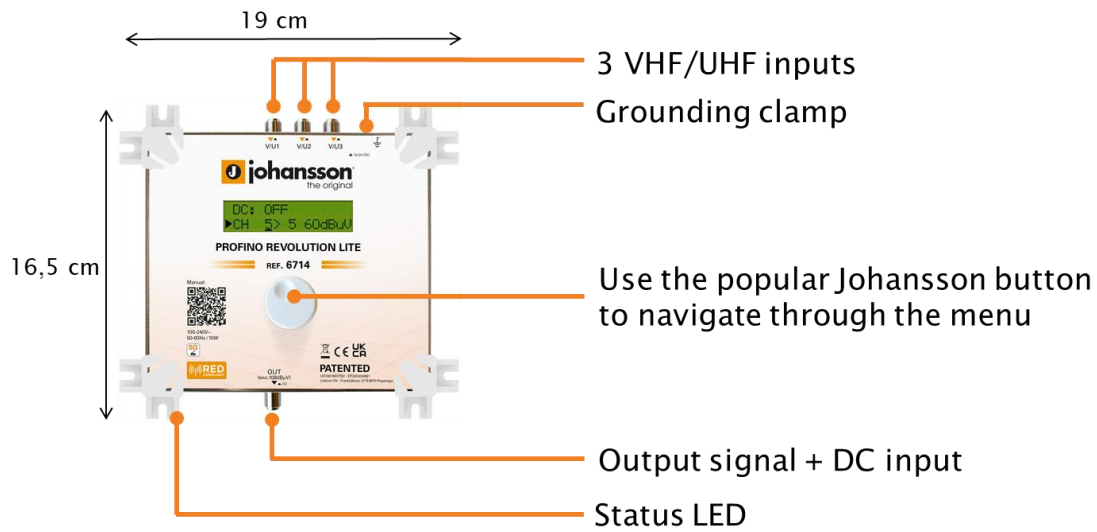
FIGURE 1: TOP VIEW OF PRODUCT
